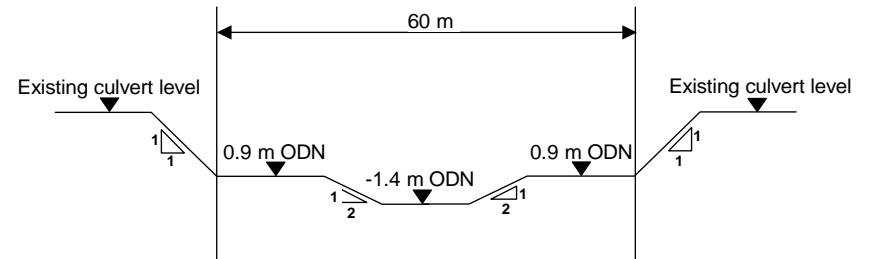
C - C Section through Breaches 1, 5, and 6
