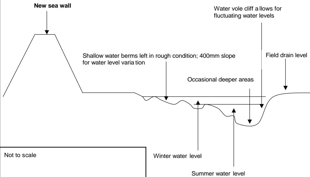
B - B Section through Wall B and Borrow Dyke B
