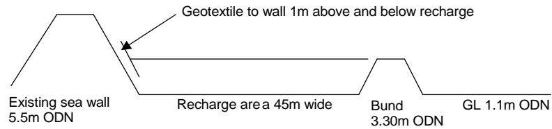
A - A Section through recharge area in front of Walls A and B
